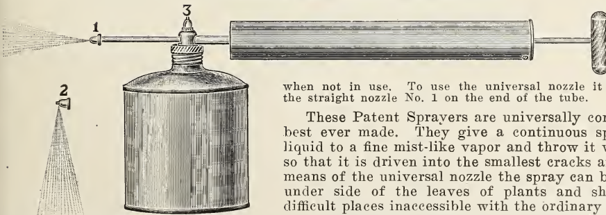
Junior No. 5 Pump.
